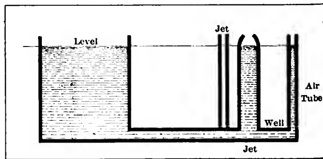
Fig. 4—Section through the Claudel carbureter, showing the well containing the jet and the compensating jet alongside
